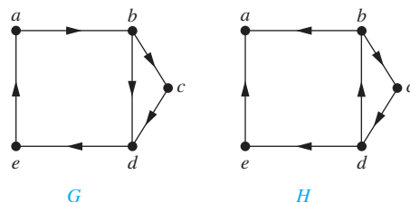
FIGURE 5 The directed graphs G and H .
