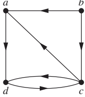
FIGURE 3 The directed graph of the relation R .
