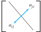
FIGURE 2 \mathbf{A} symmetric matrix.
