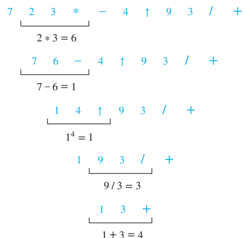
FIGURE 13 Evaluating a postfix expression.
