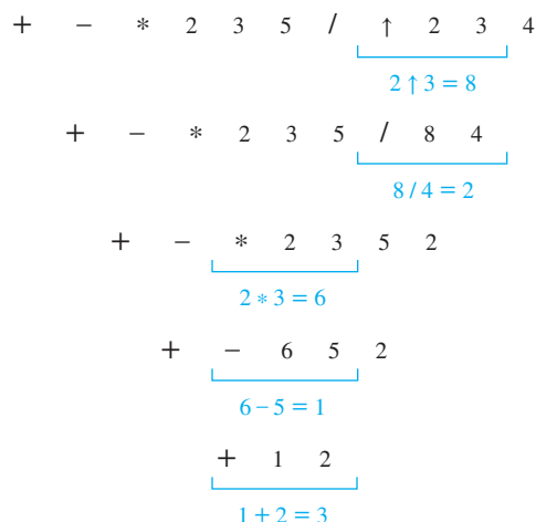
FIGURE 12 Evaluating a prefix expression.
