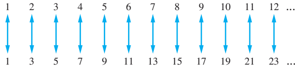
FIGURE 1 A One-to-One Correspondence Between \mathbf{Z}^+ and the Set of Odd Positive Integers.
