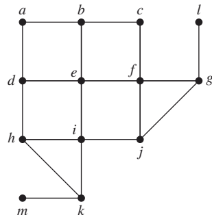
FIGURE 9 A graph G .
